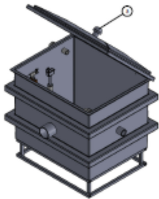
Collector-Surge Tank
